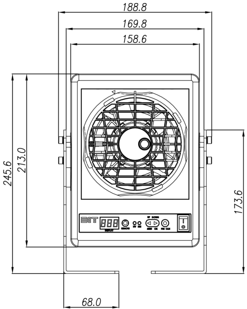
Front View
