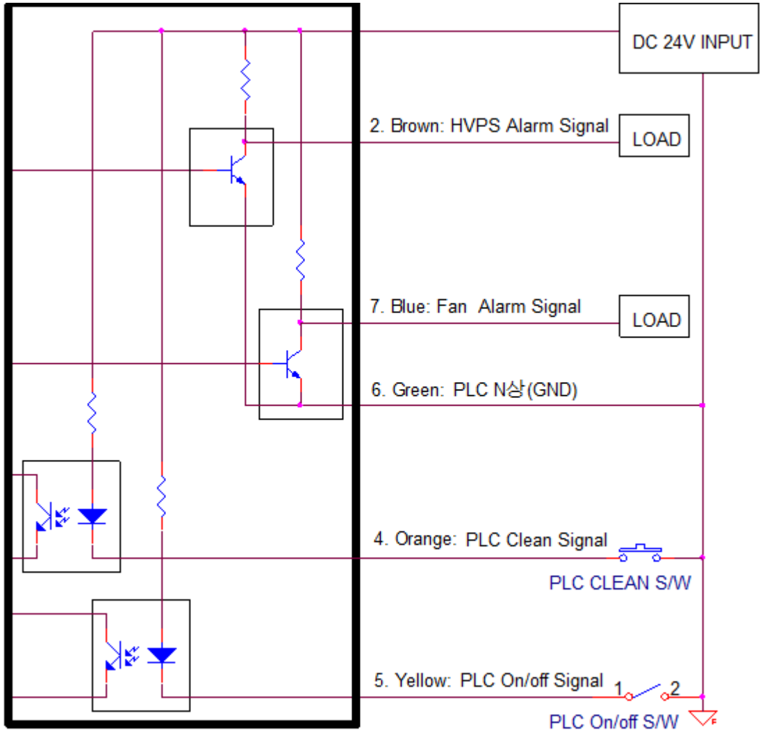
<ASF-AD/PD Series PLC(NPN Type) Circuit Diagram>
