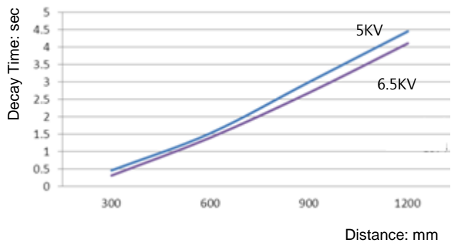
Measurement Condition : Air purge : 0.3 Mpa Charged plate dimensions : 150 x 150mm Capacity : 20pF Measure condition : 1kV -> 0.1 kV Frequency : 30Hz
