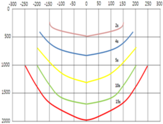
Measurement Condition : Air purge : 0.3 Mpa Charged plate dimensions : 150 x 150mm Capacity : 20pF Measure condition : 1kV -> 0.1 kV Frequency : 30Hz
