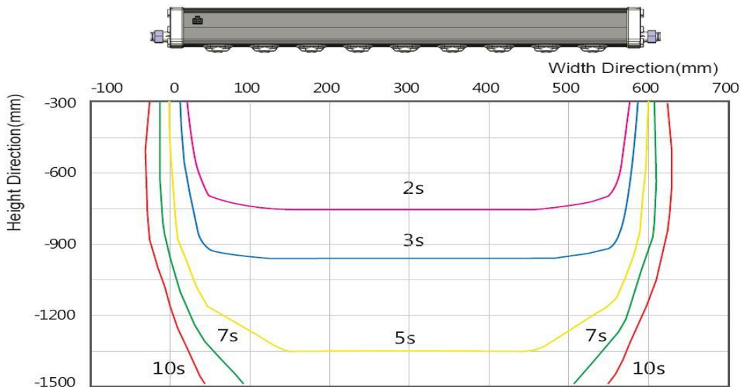
Air purge: 0.3Mpa , Capacity : 20pF , Frequency : 30Hz Charged plate dimensions : 150mm x 150mm, Measure condition : 1kV → 0.1kV
