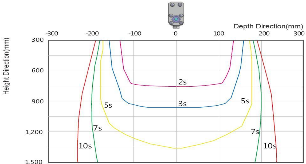
Air purge: 0.3Mpa , Capacity : 20pF , Frequency : 30Hz Charged plate dimensions : 150mm x 150mm, Measure condition : 1kV → 0.1kV
