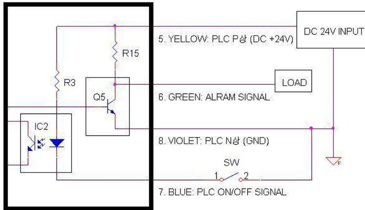
<MB-GW Series PLC Circuit Diagram>
