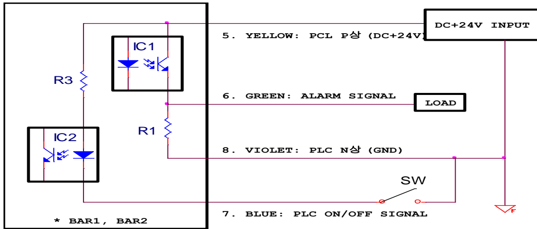
<MB-L Series PLC Circuit Diagram>
